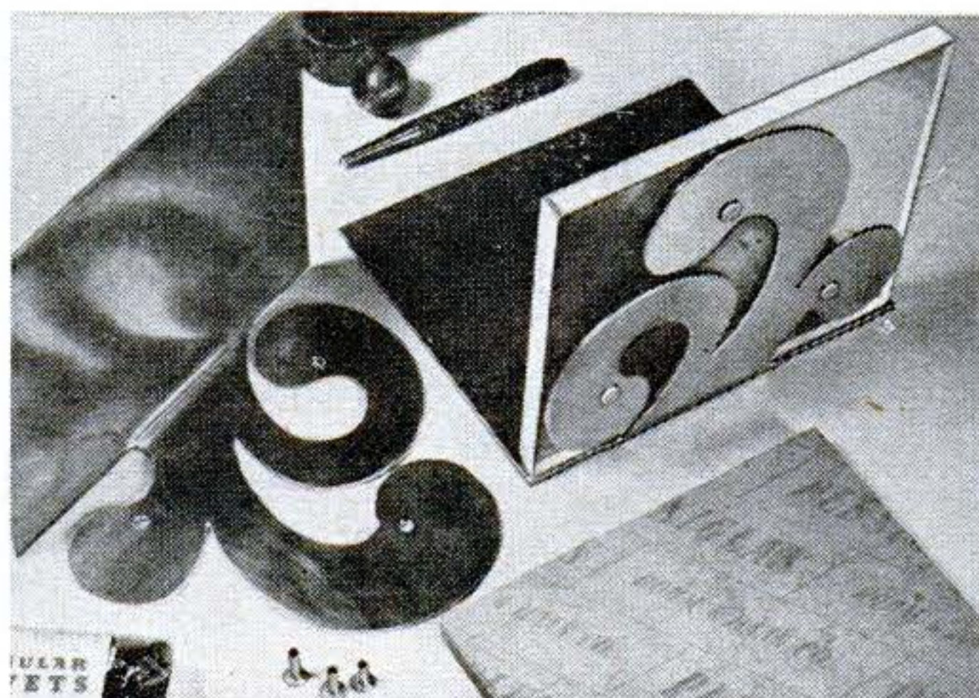
Tubular copper rivets are used to attach the copper overlay to the piece of \frac{3}{8} " clear plastic.
